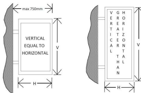
Figure 29 Dimensions for vertical projecting wall signs
